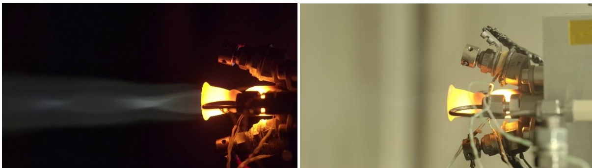
Figure 1: HyNOx-1 during steady-state operation
